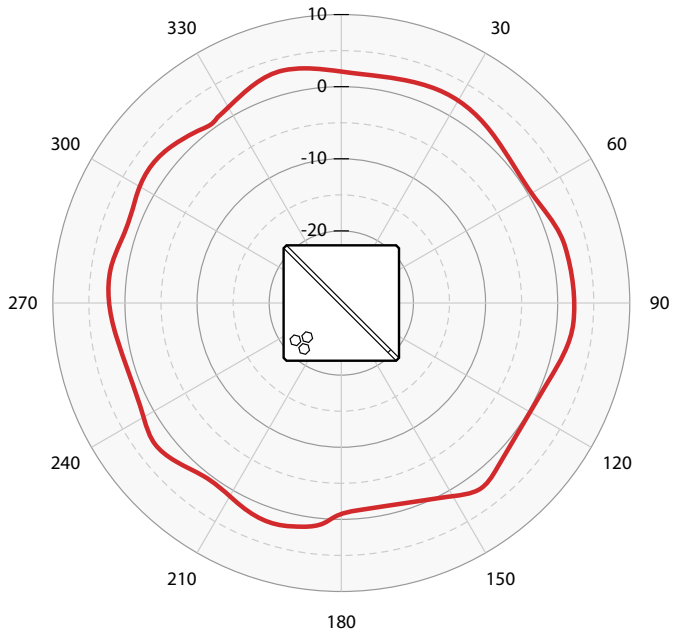
Azimuth 5 GHz
