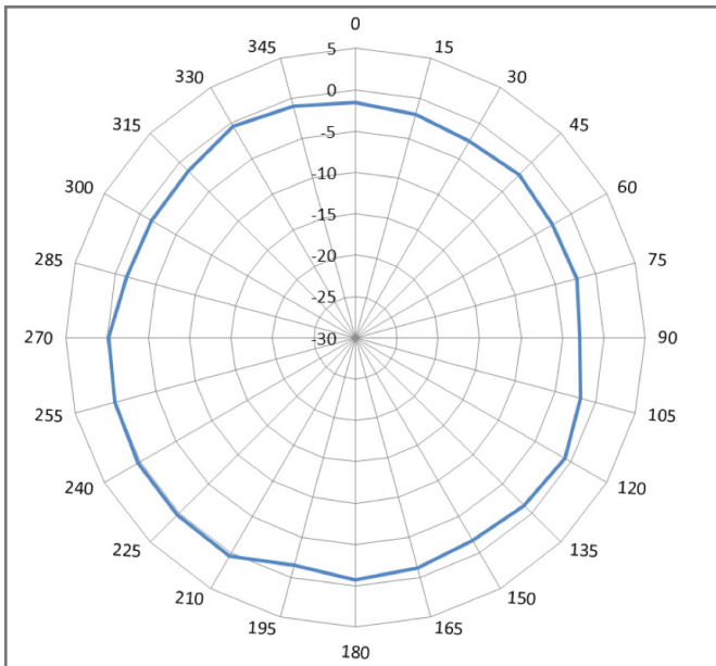
2.4GHz Horizontal/Azimuth Radiation Pattern (X-Y)
