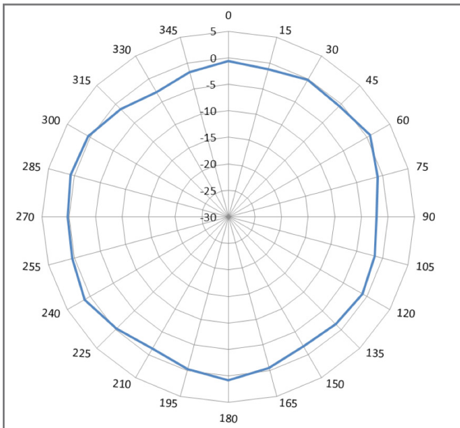
5GHz Horizontal/Azimuth Radiation Pattern (X-Y)
