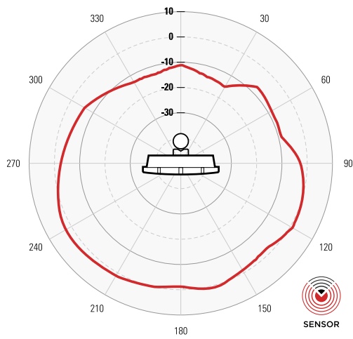
Azimuth — 5GHz
