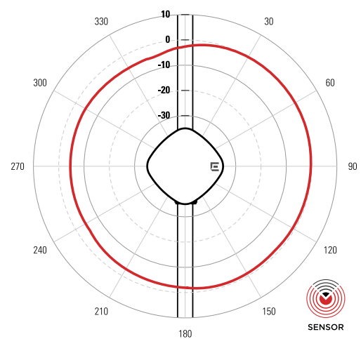
Elevation — 5GHz
