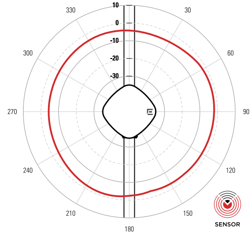
Elevation — 5GHz
